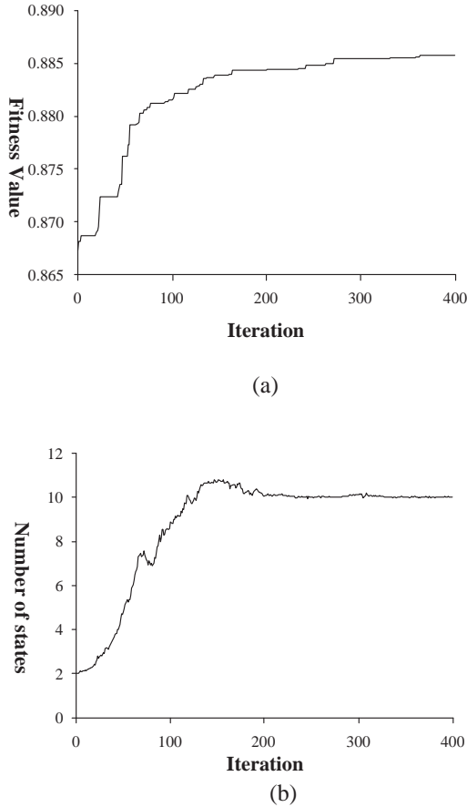
Figure 7: Results during GA-HMM training: (a) shows the fitness value of fittest individual on each iteration (b) shows average number of states for periodic signal. The GA started with a population consisting of 2 states. After 150 generations the HMM have a length of 10 states. Although the length does not significantly change thereafter the fitness continues to improve indicating that the finer structure is being fine tuned.
