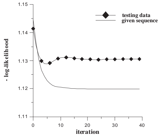
Figure 4: The graph show the negative log-likelihood for an HMM plotted against the number of Baum-Welch iterations. The negative log-likelihood for the given data is monotonically decreased by the Baum-Welch algorithm. However, the negative log-likelihood measured on independent testing data will typically decrease, reach a minimum and then increase again. In this instance the best generalisation performance was found after 5 iterations. The training data used was from C. jejuni and is described in experiment I below.
