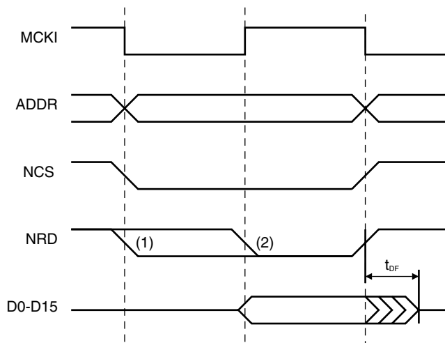
Figure 18. Data Float Output Time
